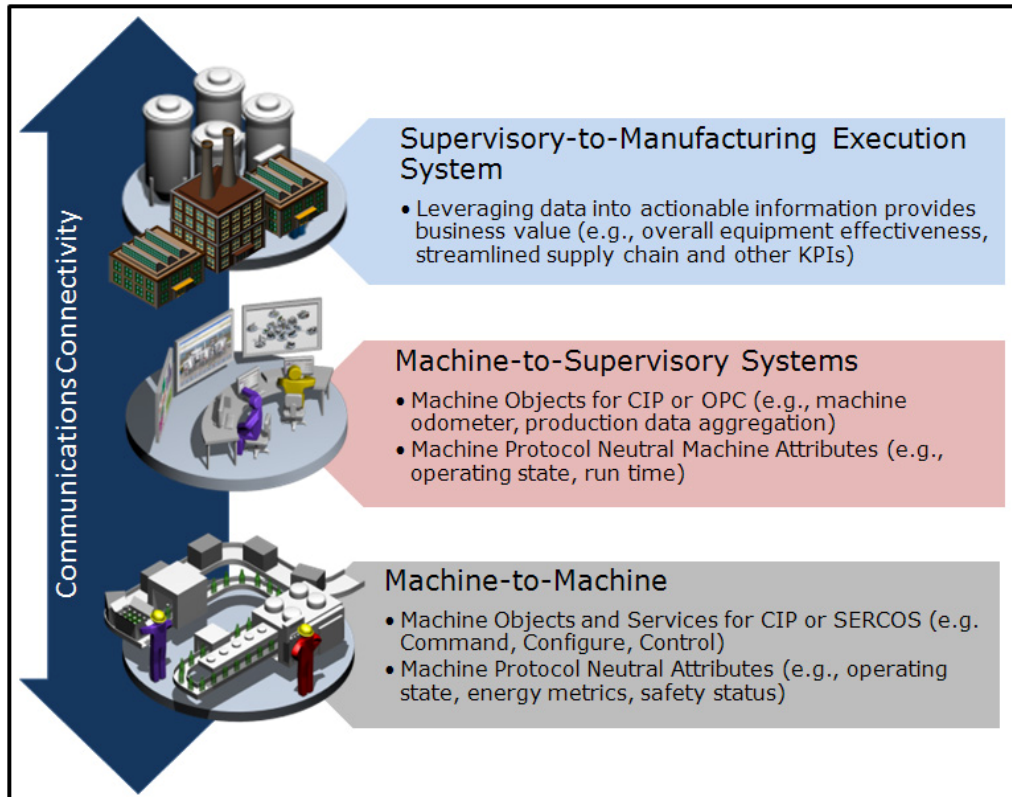
Figure 3. The Unified Integration Model across all three levels of the production domain
